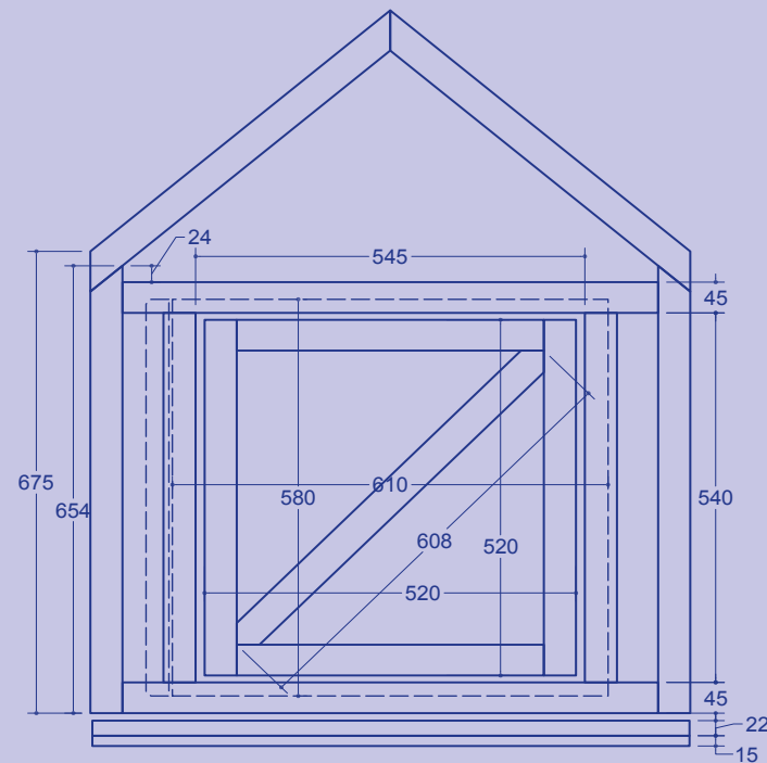
Section showing back frame 1 : 12
