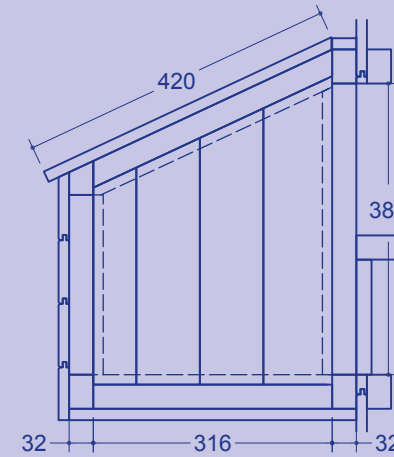
Section through divider in nest box 1 : 10
