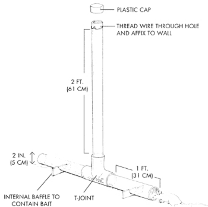
Rodent bait station
